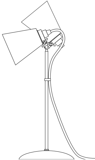
FT429N Hector Medium Flowerpot Table Light, Natural H: 460 mm x W: 240 mm (as photographed) H: 570 mm, W: 240 mm (maximum)
